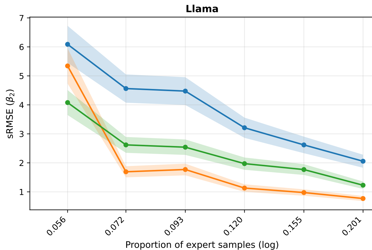
Low-Variance Feature — sRMSE of \beta_2 (MISOGYNISTIC)
